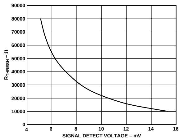
Figure 5. Signal Detect Voltage vs. R_{THRESH}
